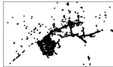
Figure 4(a): Spatial plot of sample data before clustering
